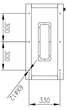
BOTTOM VIEW
