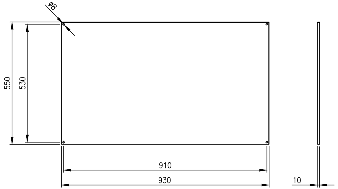
DEVICE MOUNTING PLATE
