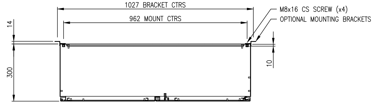
SECTION AW-AW
