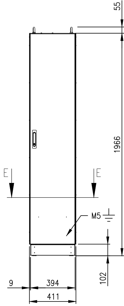
FRONT VIEW (ASSEMBLY)
