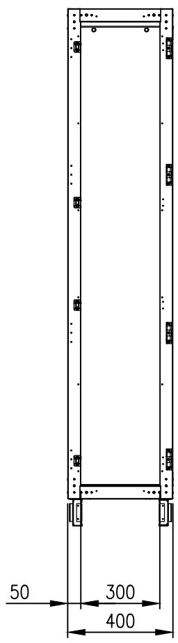
FRONT VIEW (PANELS REMOVED)
