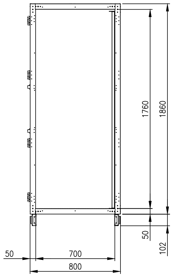
SIDE VIEW (PANELS REMOVED)
