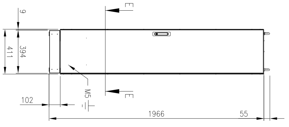
FRONT VIEW (ASSEMBLY)
