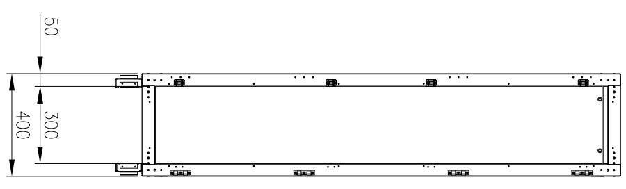
FRONT VIEW (PANELS REMOVED)
