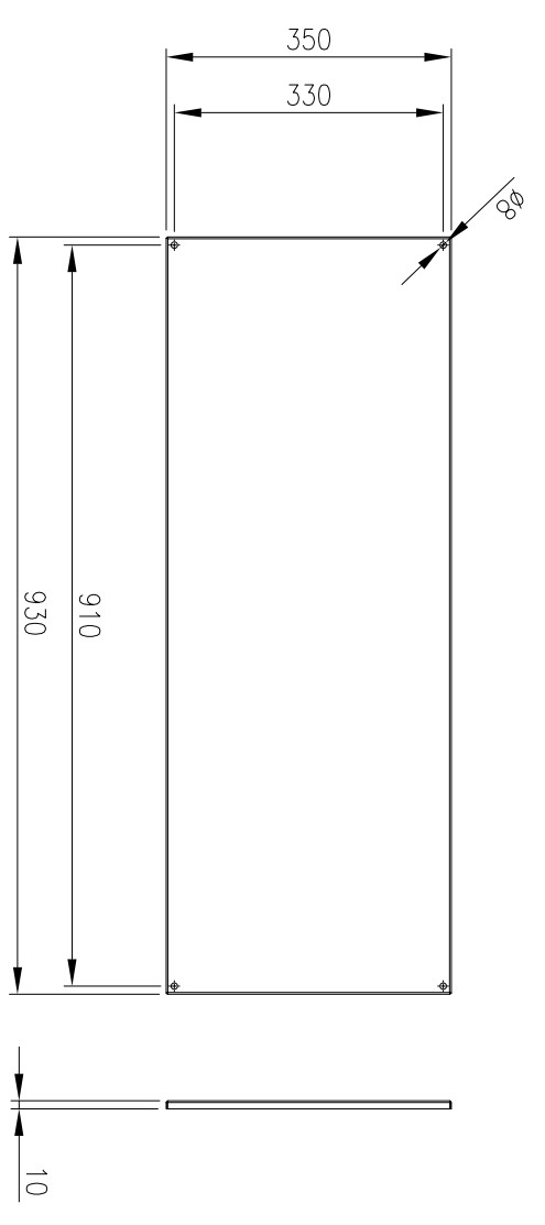
DEVICE MOUNTING PLATE
