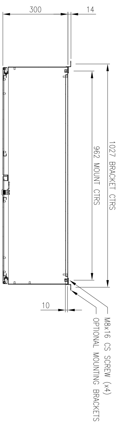
SECTION AW-AW
