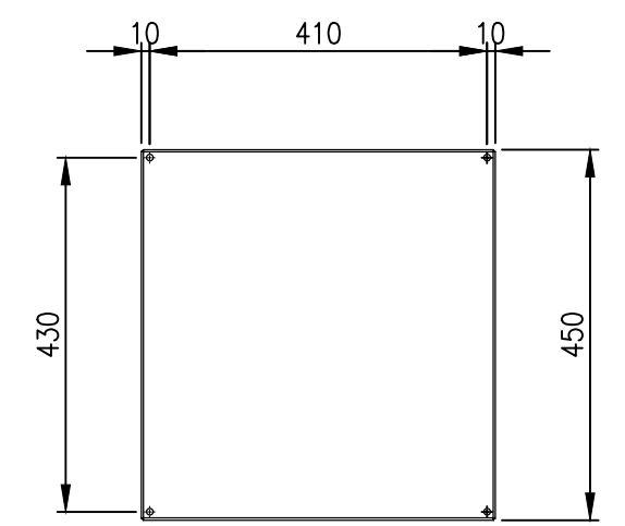
MOUNTING PLATE (PAINTED TO RAL9010)
